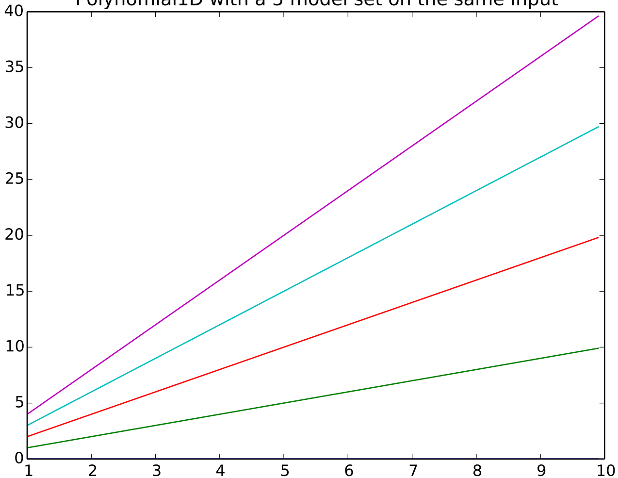
Polynomial1D with a 5 model set on the same input
