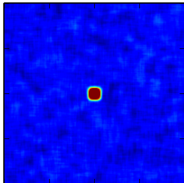
Box2DKernel
