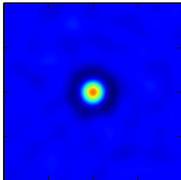
MexicanHat2DKernel
