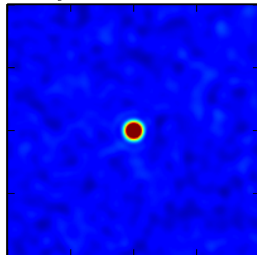
AiryDisk2DKernel
