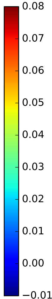
AiryDisk2DKernel
