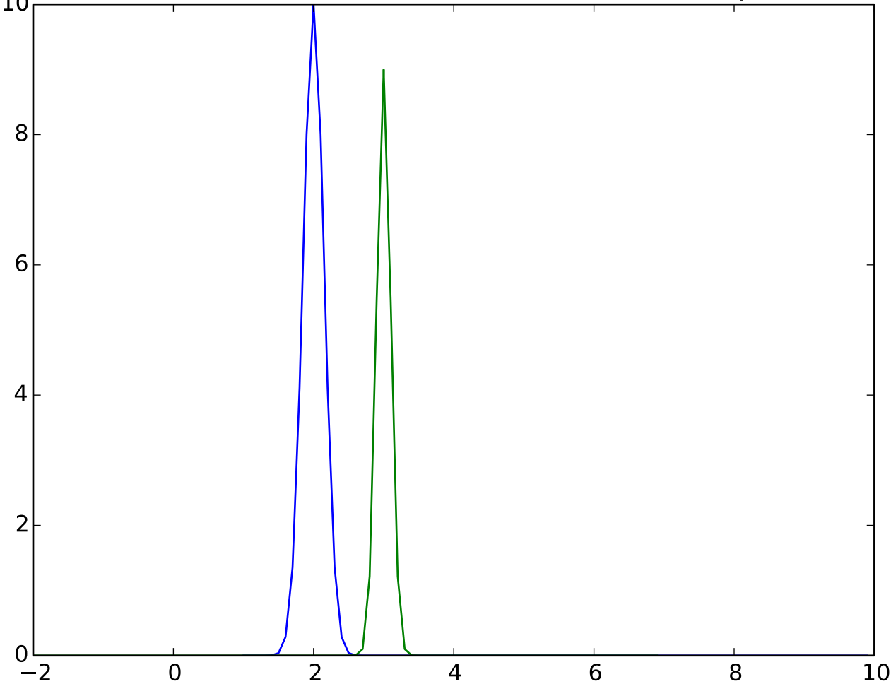
Evaluate two Gaussian1D models with 2 sets of input data
